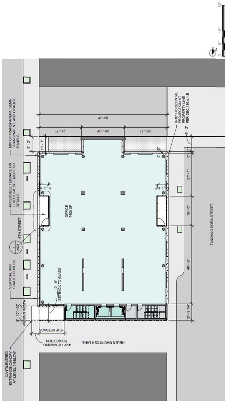
Figure 4. Typical Levels 2, 4, and 6 Plan
